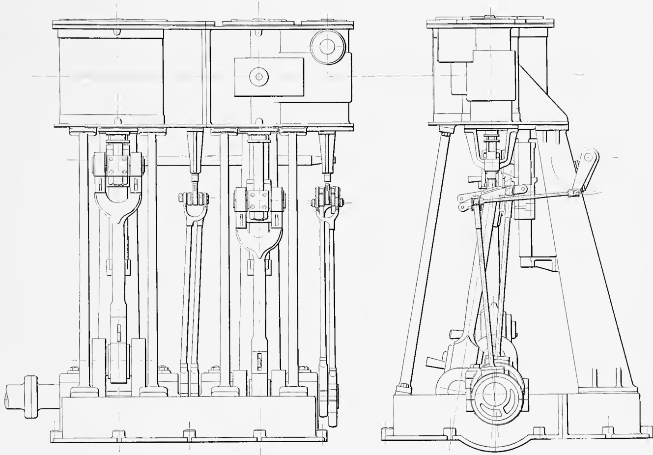
COMPOUND ENGINES OF BOSTON'S NEW FIRE BOAT.—Built by Brown &amp; Miller, Jersey City, N. J.
